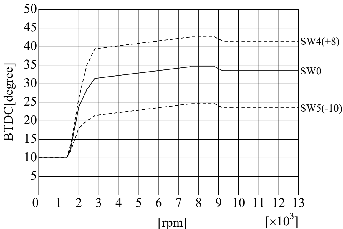
SP2FPKit (H.CBX400F) ignition curve AS UOTANI
