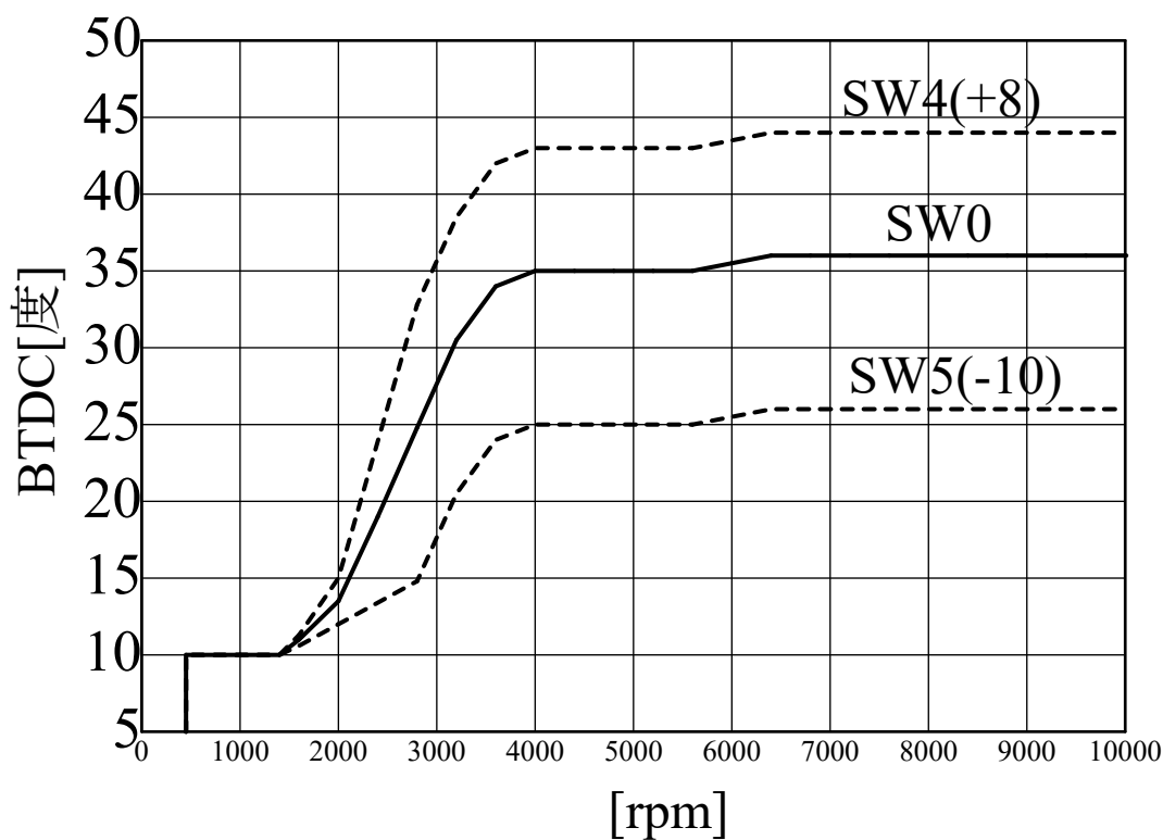
SP2FPKit(H.CB750K) ignition curve
