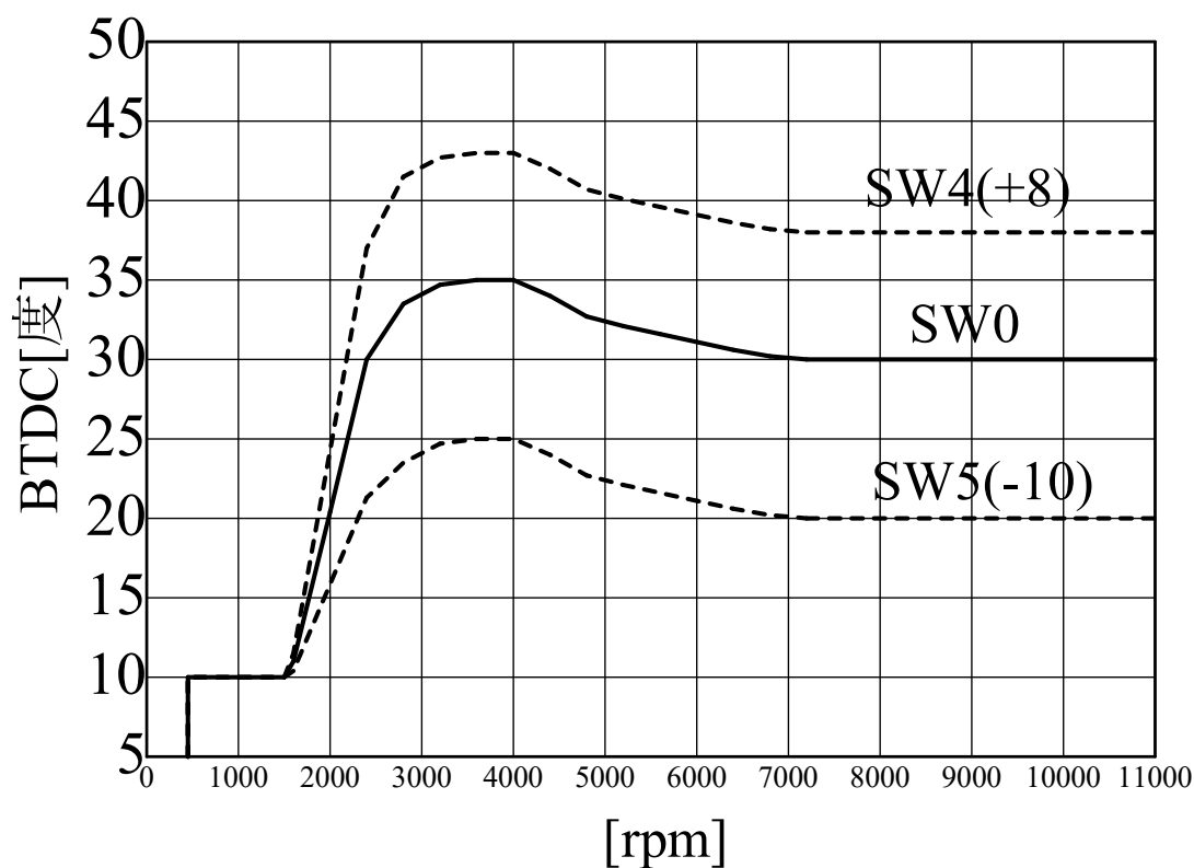
SP2FPKit(H.CB400F) ignition curve
