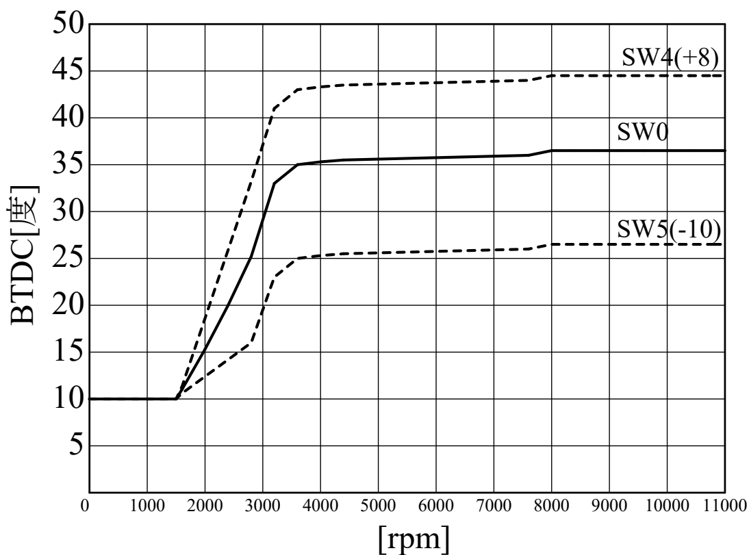
SP2FPKit (H.CBX750F) ignition curve AS UOTANI
