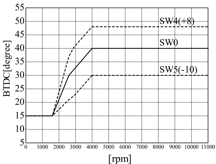
SP2FPKit(H.CB400T/N) ignition curve
