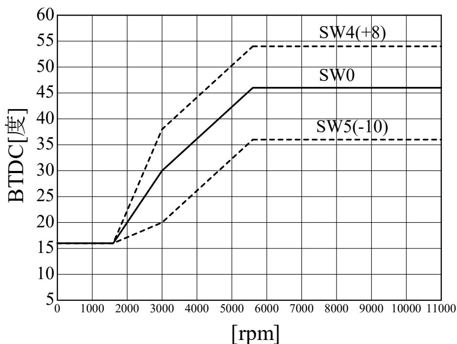
SP2FPKit(H.CB250T/N) ignition curve
