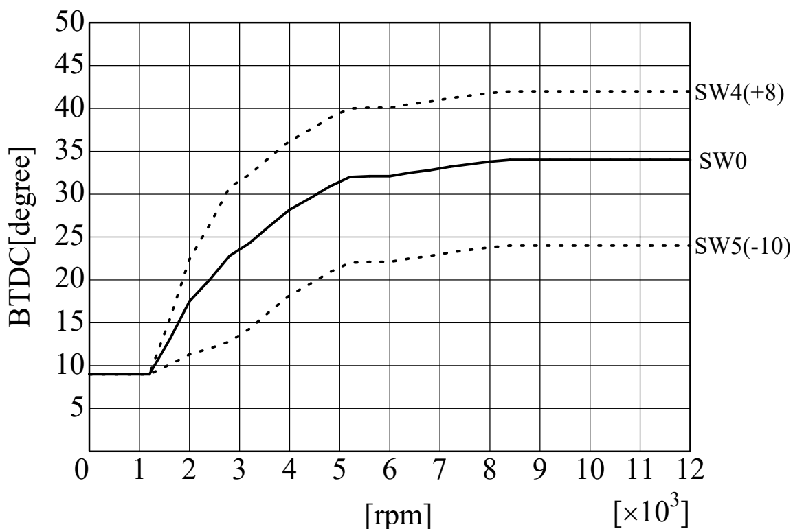
SP2FPKit (H.CB750F) ignition curve AS UOTANI
