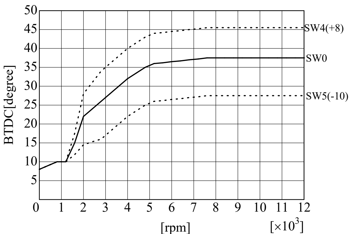
SP2FPKit (Y.FZ750) ignition curve AS UOTANI
