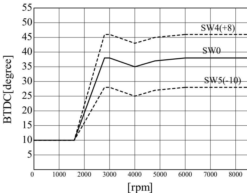
SP2FPKit (Y.XS650-1) ignition curve AS UOTANI
