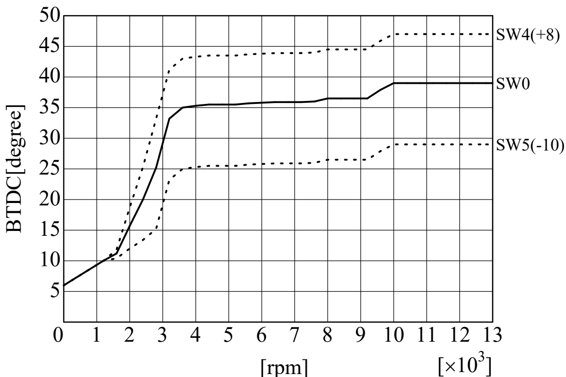
SP2FPKit (K.GPZ1000RX) ignition curve AS UOTANI
