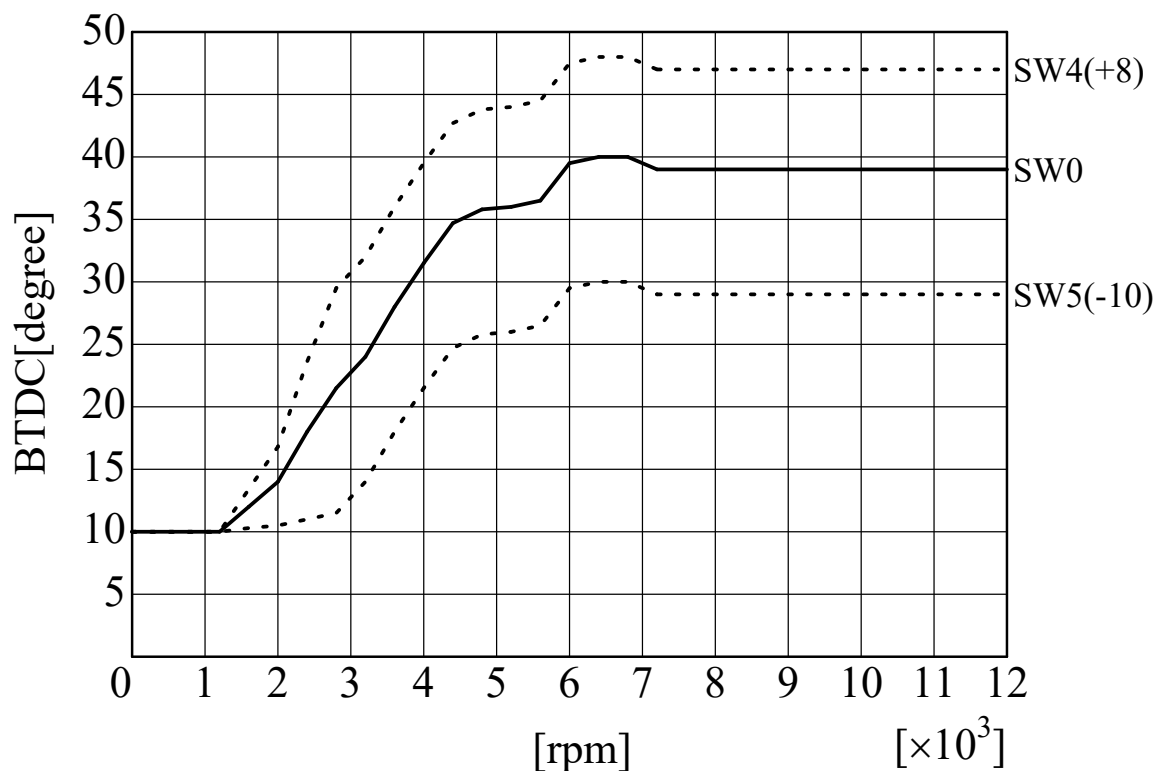
SP2FPKit (K.GPZ1100E) ignition curve AS UOTANI
