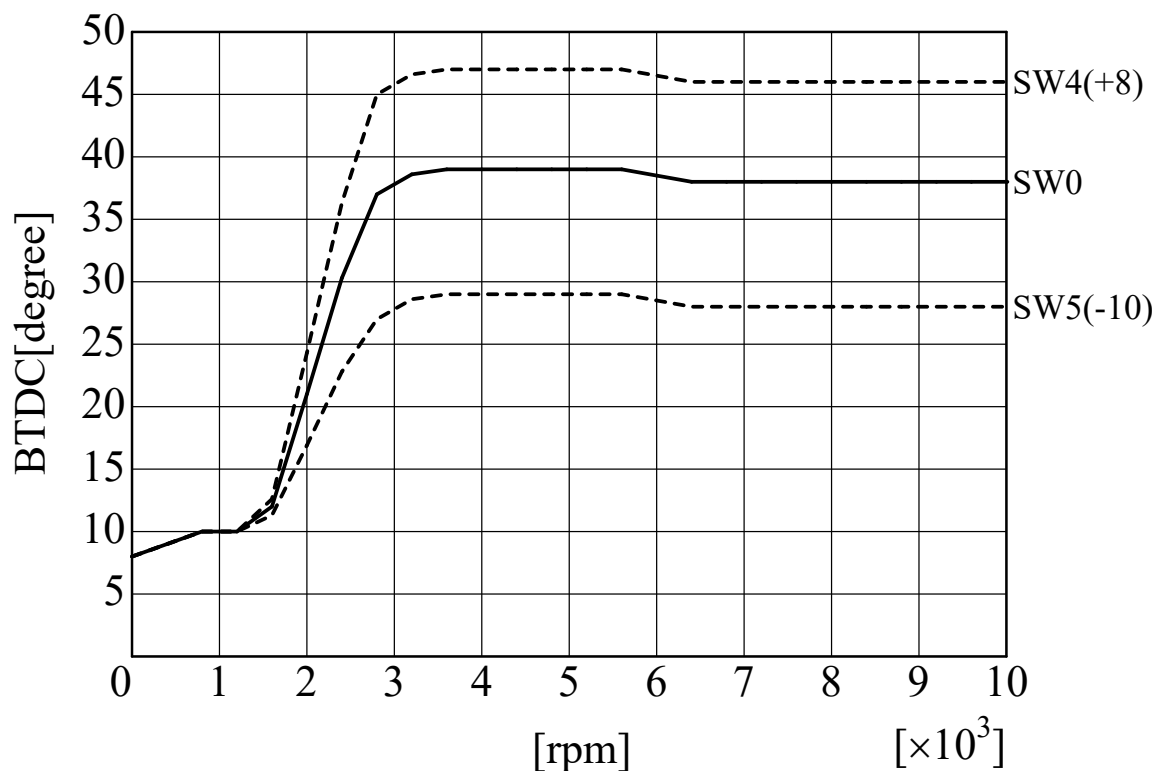
SP2FPKit (K.KZ1300) ignition curve AS UOTANI
