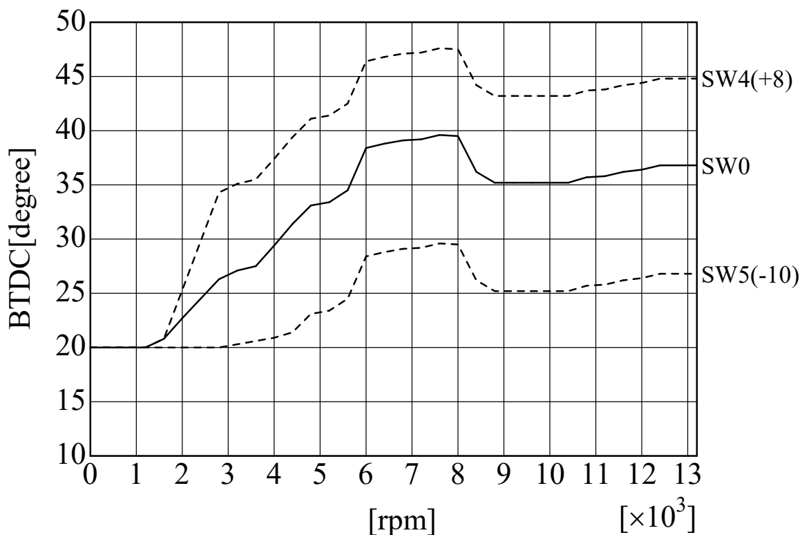
SP2FPKit (K.ZRX400-1) ignition curve AS UOTANI
