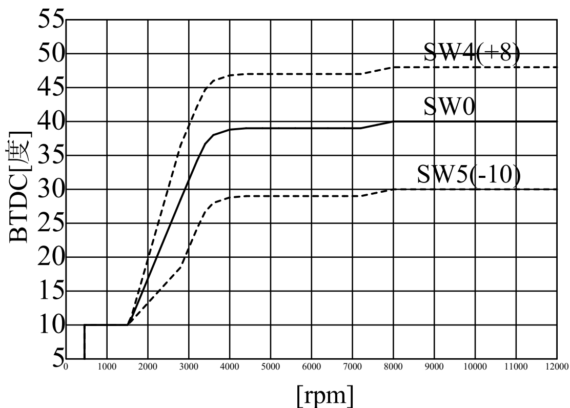
SP2FPKit(K.Z750FX2) ignition curve
