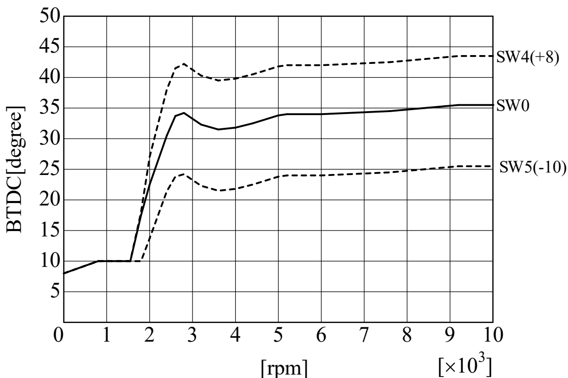
SP2FPKit (K.KZ1300-2) ignition curve AS UOTANI
