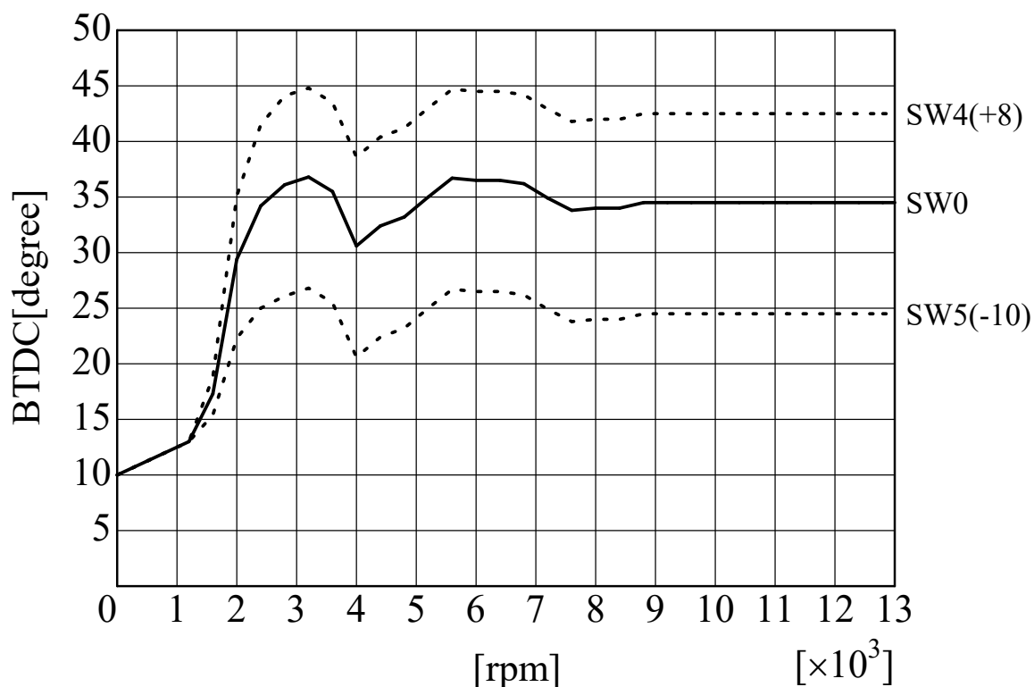
SP2FPKit (S.GSX-R1100-1) ignition curve AS UOTANI
