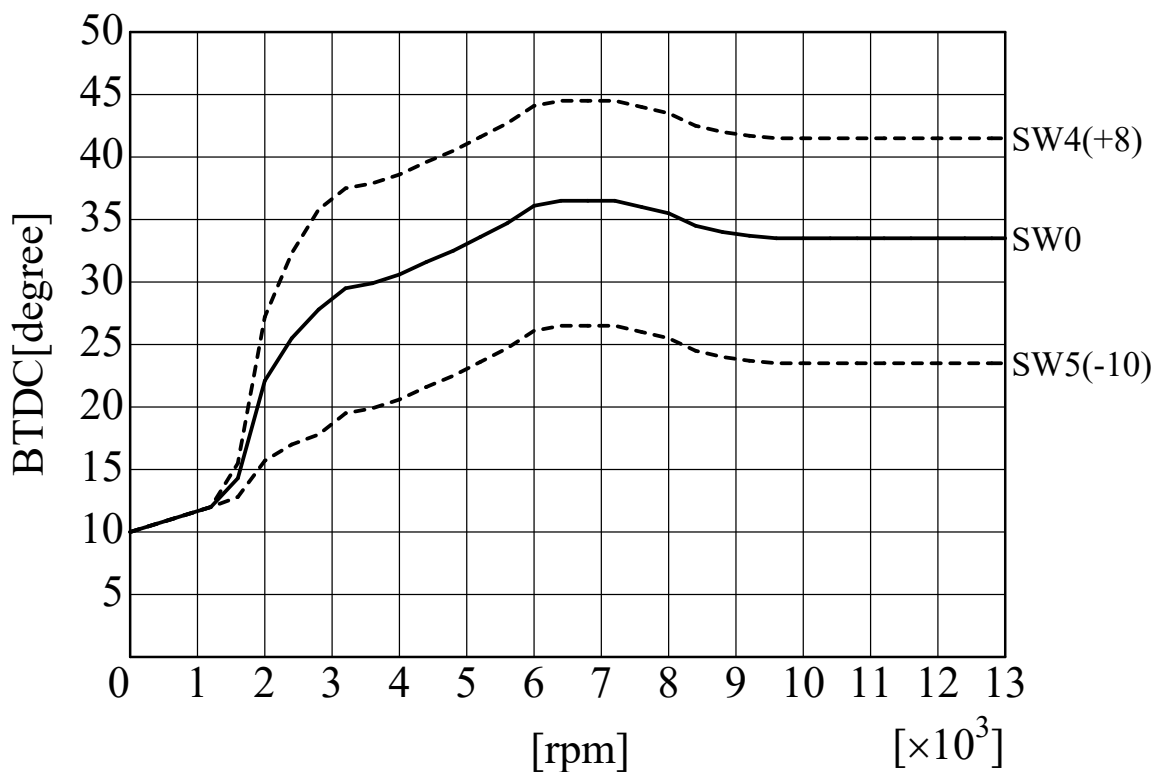
SP2FPKit (S.GSX-R1100-2) ignition curve AS UOTANI
