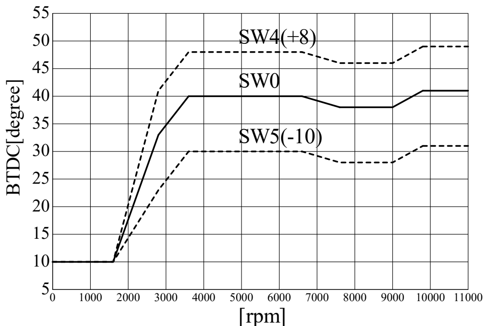
SP2FPKit(S.GSX400F) ignition curve
