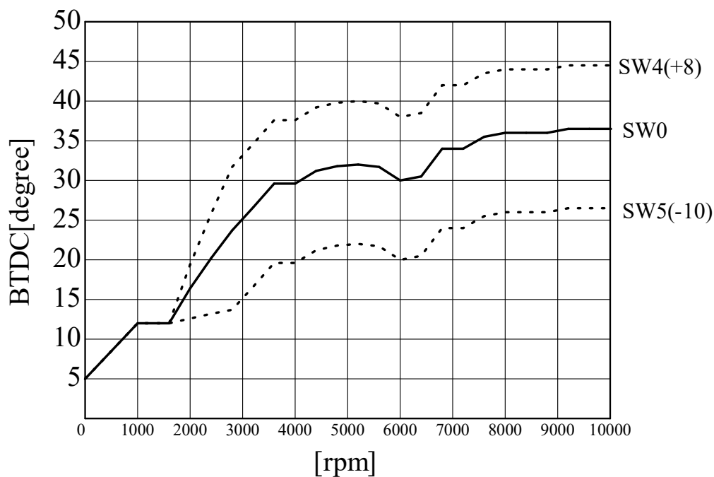
SP2FPKit (S.GSX1100S) ignition curve AS UOTANI
