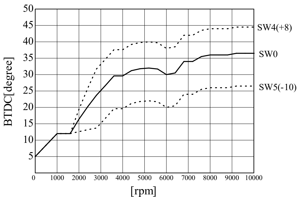
SP2FPKit (S.GSX750E) ignition curve AS UOTANI
