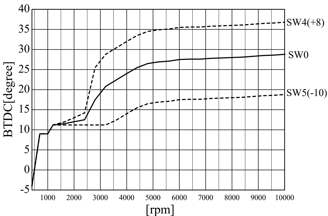
SP2FPKit (D.900HHR/SS) ignition curve AS UOTANI
