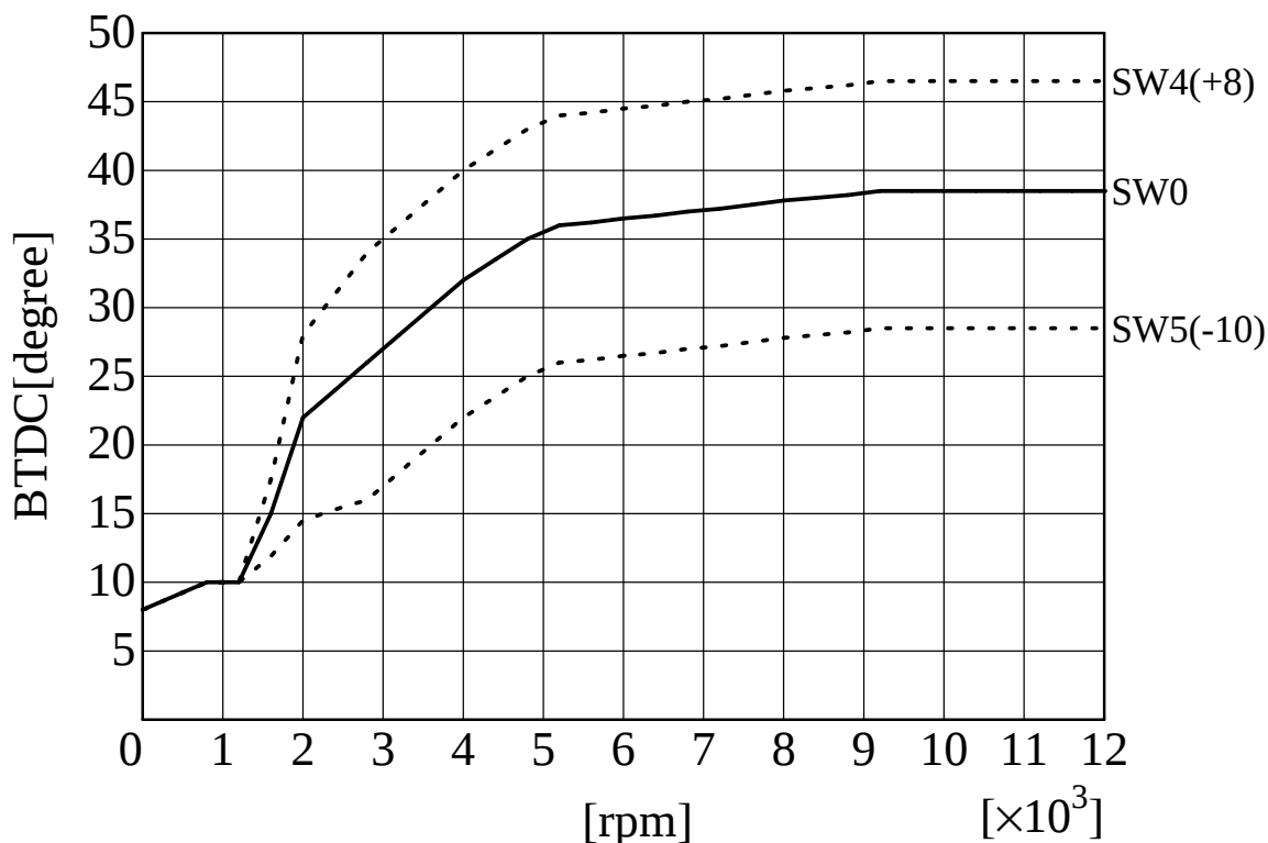
SP2FPKit (H.CBX1000) ignition curve AS UOTANI
