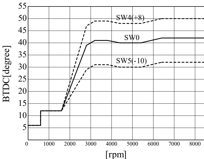
SP2FPKit (Y.XS650-2) ignition curve AS UOTANI
