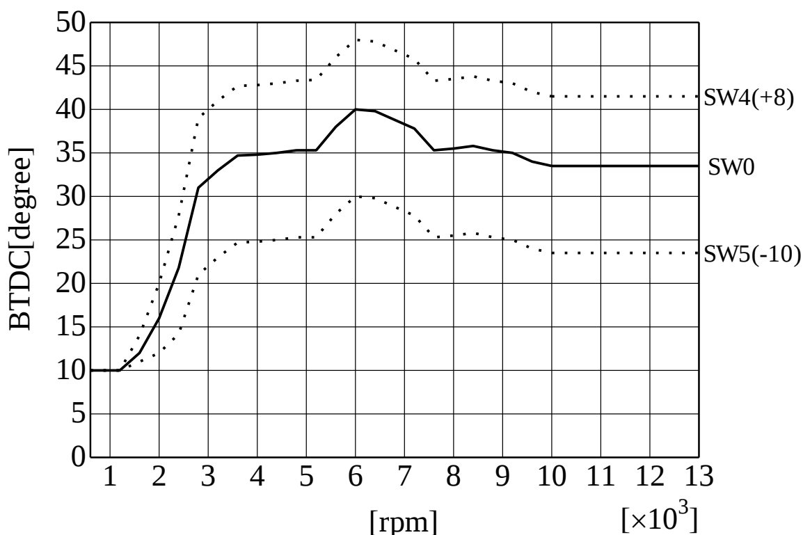
SP2FPKit (K.ZZR1100C) ignition curve AS UOTANI
