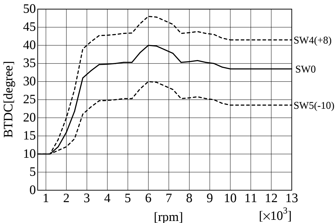
SP2FPKit (K.ZZR1100D) ignition curve AS UOTANI
