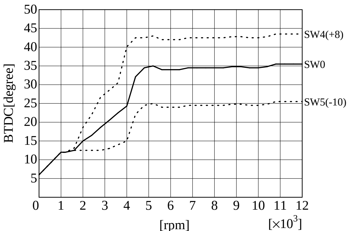
SP2FPKit (K.ZEPHYR750) ignition curve AS UOTANI
