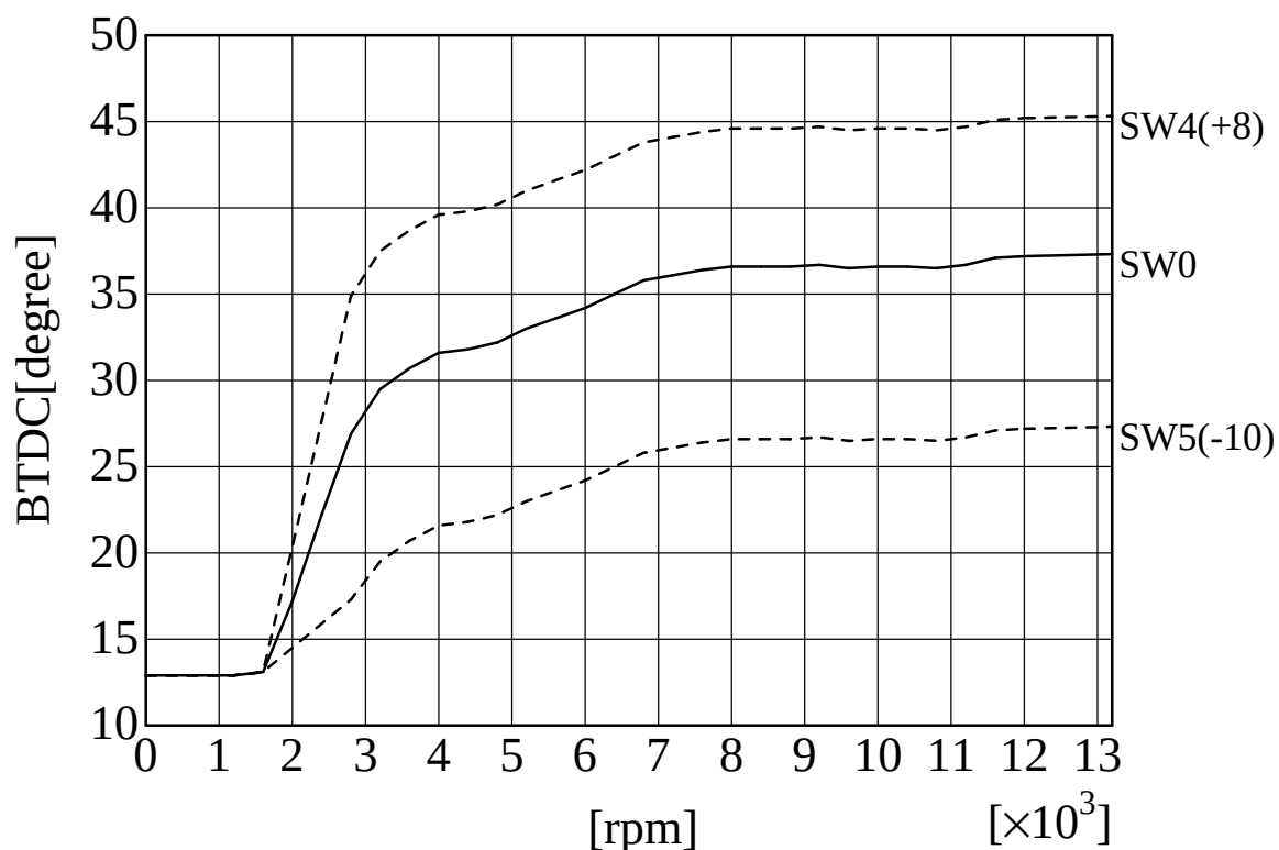
SP2FPKit (ZEPHYR400) ignition curve AS UOTANI
