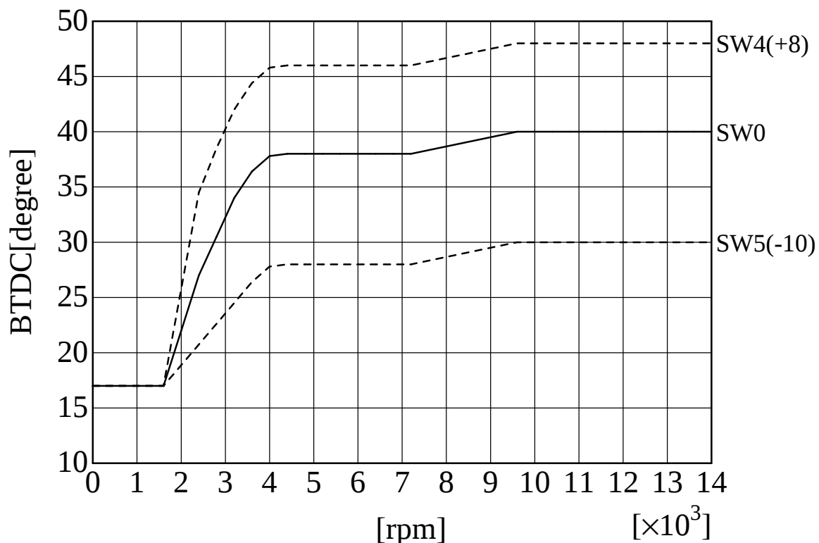
SP2FPKit (GPZ400R-1) ignition curve AS UOTANI
