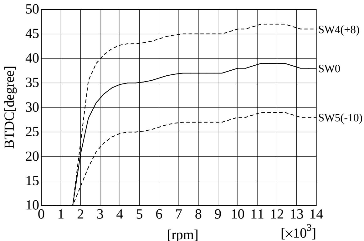
SP2FPKit (GPZ400R-2) ignition curve AS UOTANI
