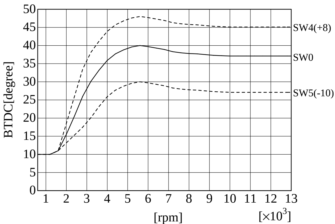
SP2FPKit (ZX-10) ignition curve AS UOTANI
