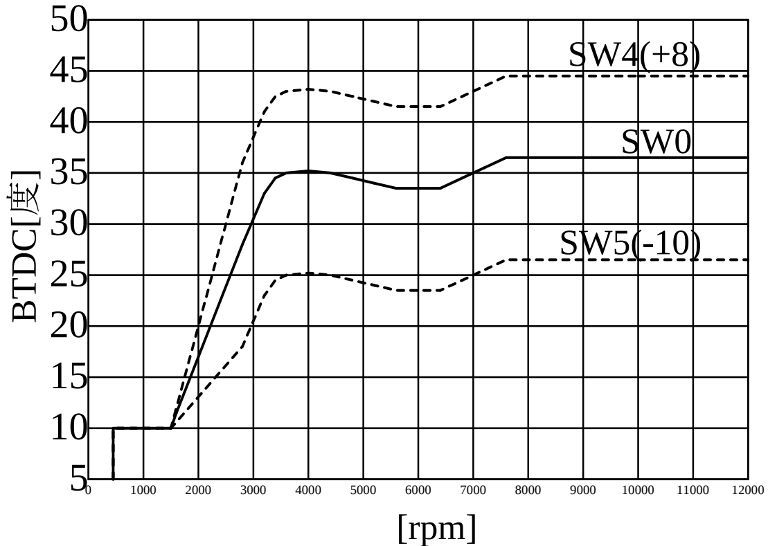
SP2FPKit(K.Z400FX) ignition curve
