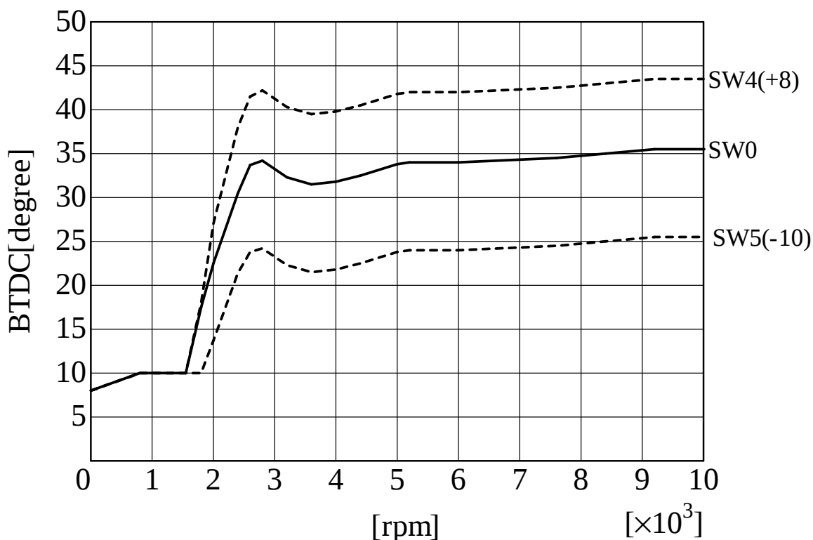
SP2FPKit (K.KZ1300A3) ignition curve AS UOTANI
