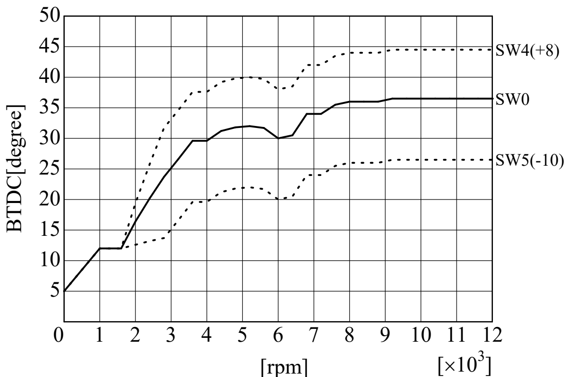
SP2FPKit (S.GSX1100S) ignition curve AS UOTANI
