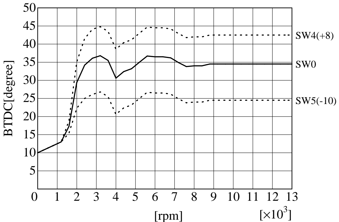
SP2FPKit (S.GSX-R1100-1) ignition curve AS UOTANI
