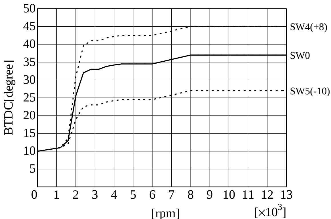
SP2FPKit (S.GSX-R1100J) ignition curve AS UOTANI
