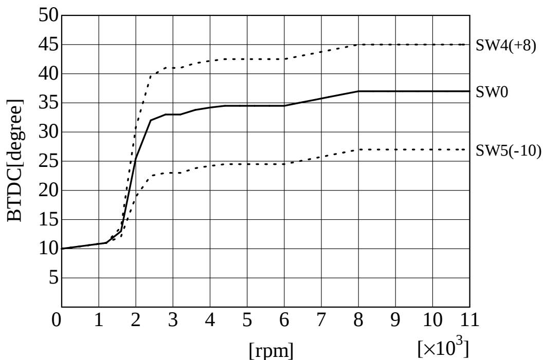
SP2FPKit (S.GSX750S-3) ignition curve AS UOTANI
