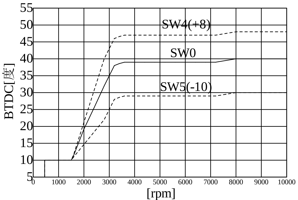
SP2FPKit(GS400) ignition curve
