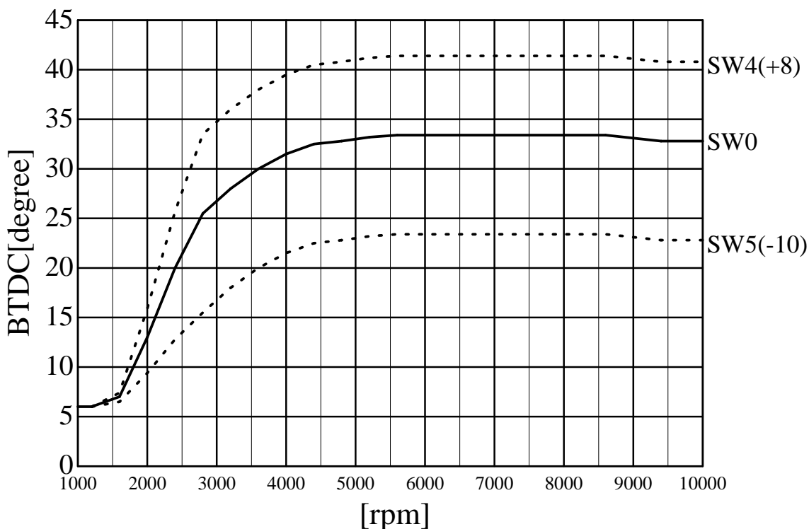
SP2FPKit (D.M900/SS) ignition curve AS UOTANI
