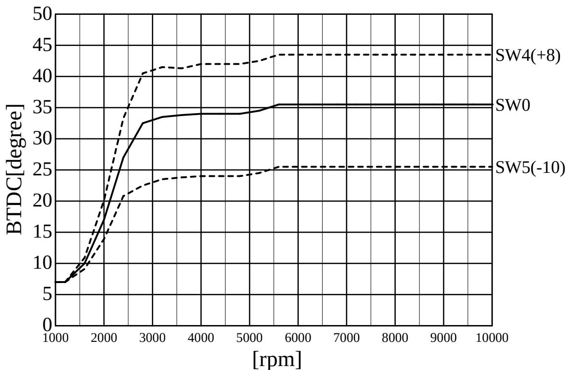
SP2FPKit (D.750F1-K) ignition curve AS UOTANI
