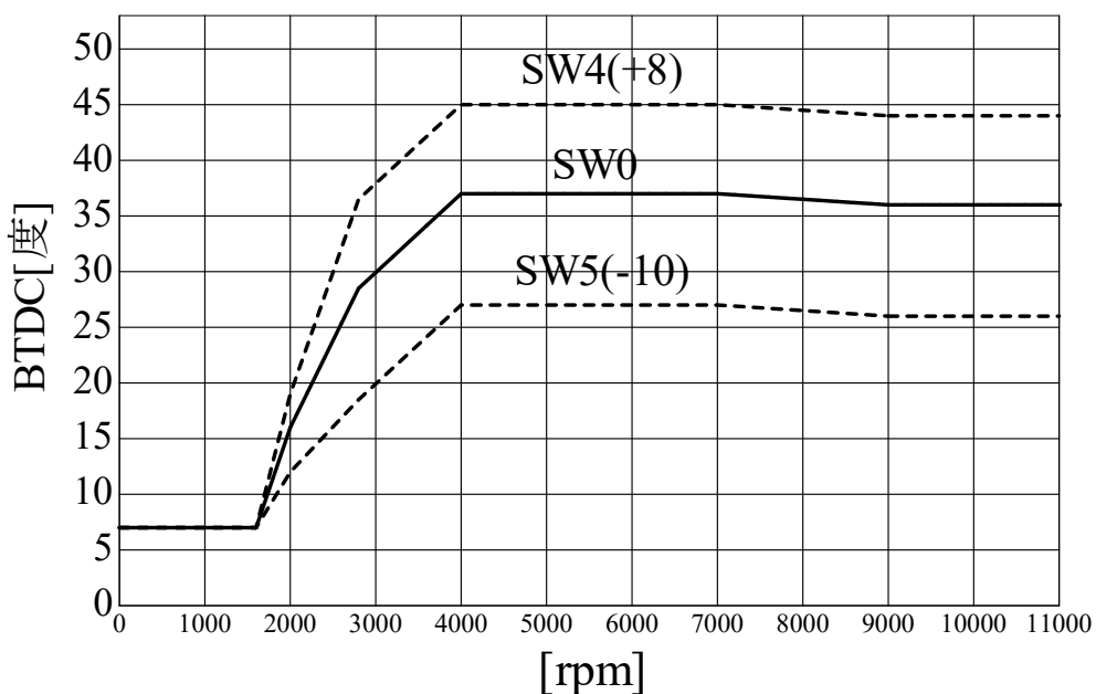
SP2FPKit(Y.XJ750E) ignition curve
