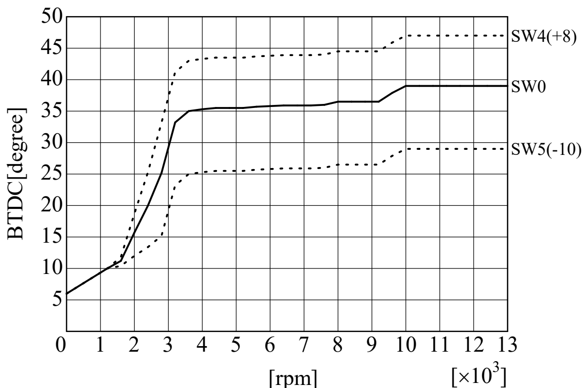
SP2FPKit (K.GPZ900R-1) ignition curve AS UOTANI
