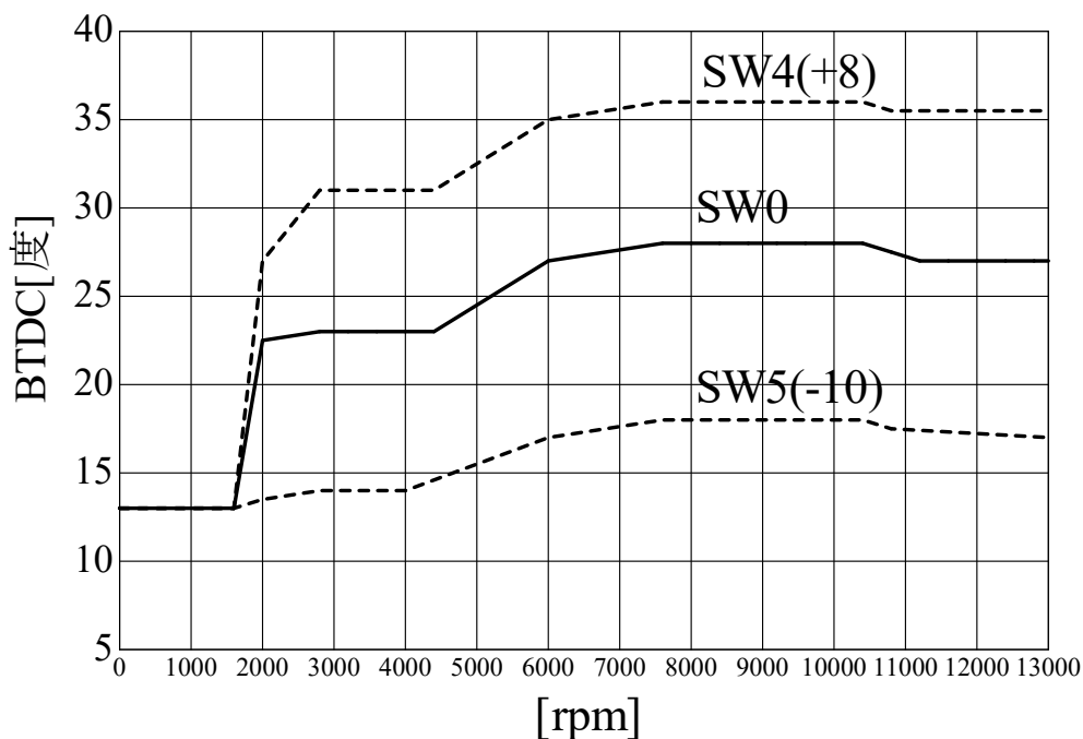
SP2FPKit(S.INAZUMA400) ignition curve (GK7BA-100001 ~ TPS無し車)
